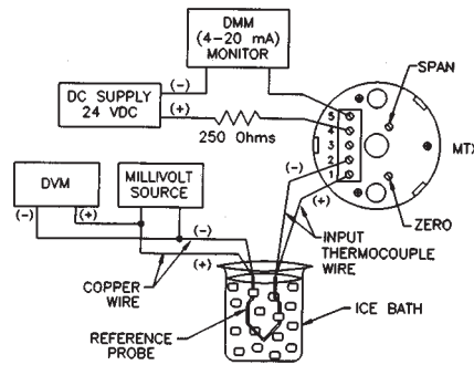
Figure 4-1. Calibration Setup Using a Millivolt Source
