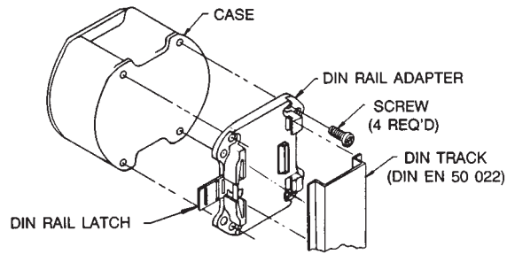
Figure 3-3 DIN Track Mounting
