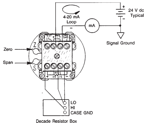
Figure 5-1 Calibration Setup
