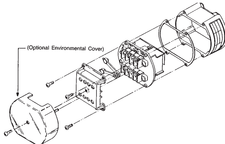
Figure 3-1 Exploded View of Model 501
