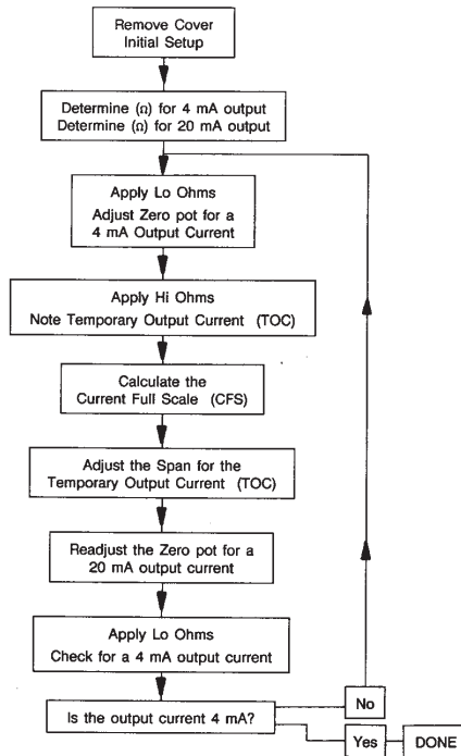
Figure 5-2 Calibration Flowchart
