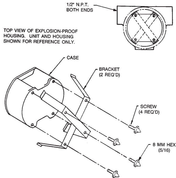
Figure 3-4 Spring Retainer for Explosion-Proof Housing
