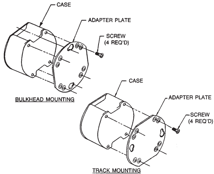
Figure 3-2 Bulkhead and Track Mounting
