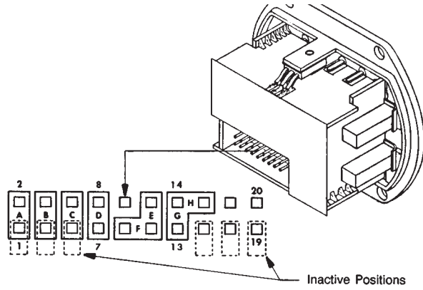
Figure 5-3 Jumper Diagram
